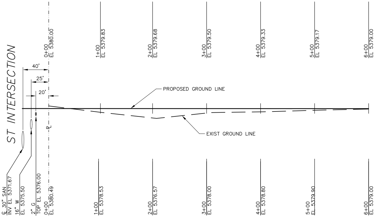
TYPICAL STREET CL PROFILE
