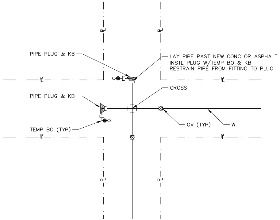
FOUR-WAY INTERSECTION
