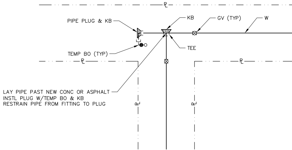
THREE-WAY INTERSECTION
