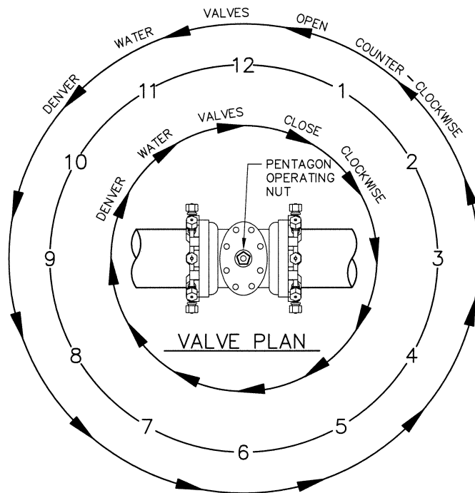
RECYCLED VALVE OPENING & CLOSING DIRECTION
