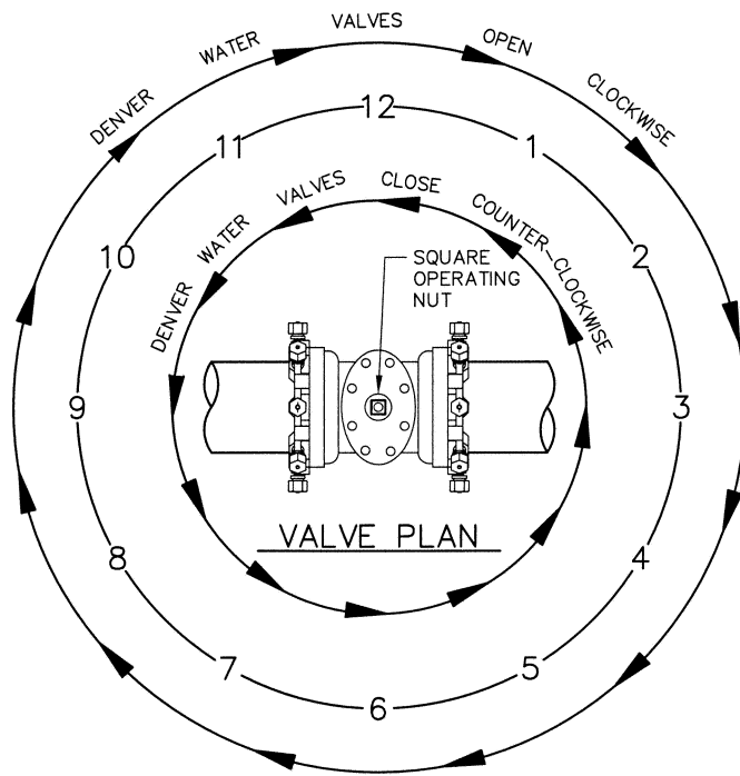
TREATED/POTABLE VALVE OPENING & CLOSING DIRECTION
