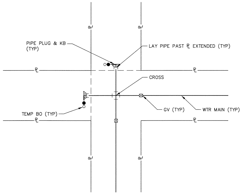
FOUR-WAY INTERSECTION
