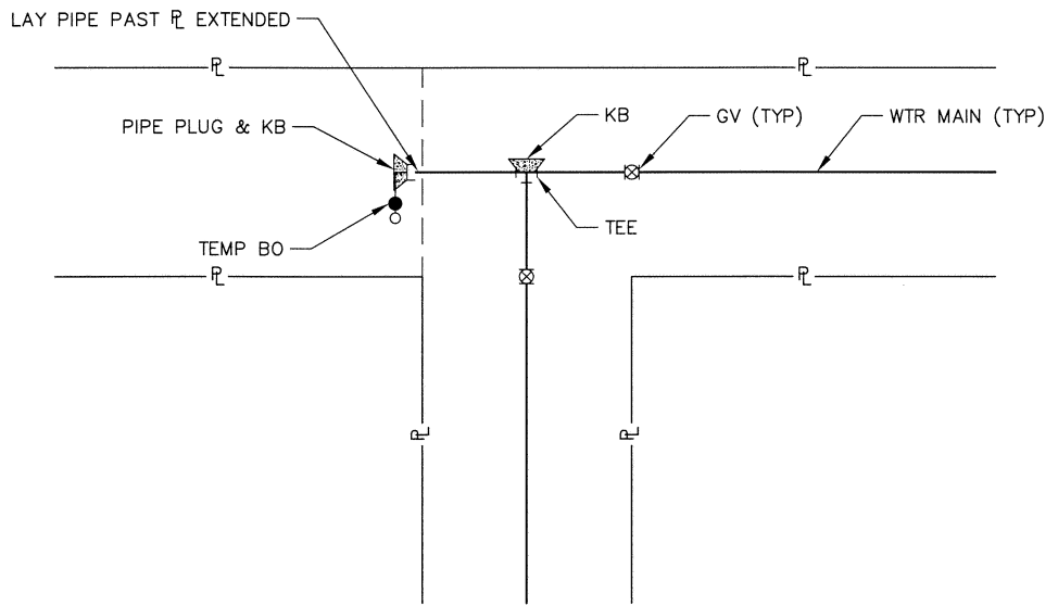
THREE-WAY INTERSECTION
