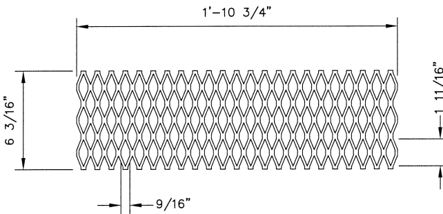
METAL SCREEN
