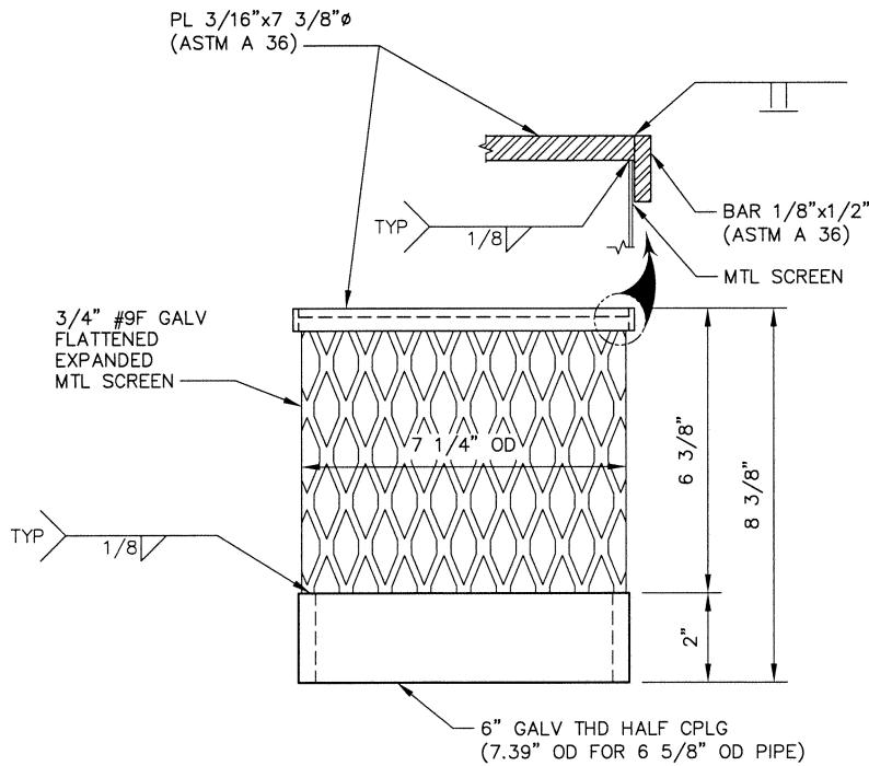
VENT SCREEN ASSEMBLY
