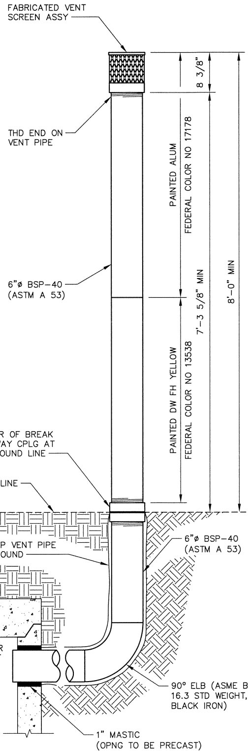
VENT PIPE ELEVATION
